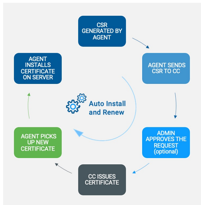
Automated certificate provisioning with CertCentral® Managed Automation
