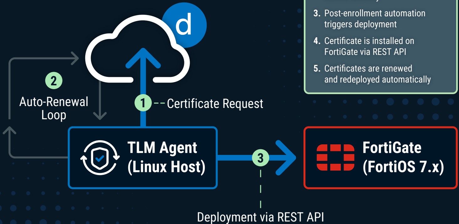
Figure 1: Automated certificate lifecycle workflow between DigiCert Trust Lifecycle Manager and FortiGate
